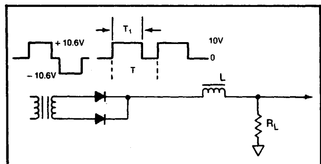
Figure 7-104. A13 Regulator, Simplified Schematic
