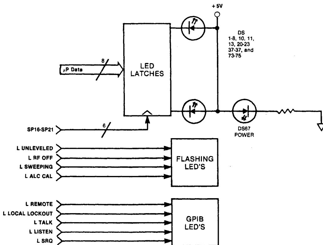
Figure 7-19. All Front Panel PCB, Block Diagram
