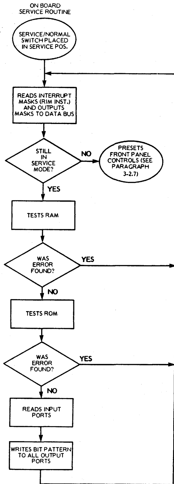
Figure 7-17. A12 PCB On-Board Service Routine
