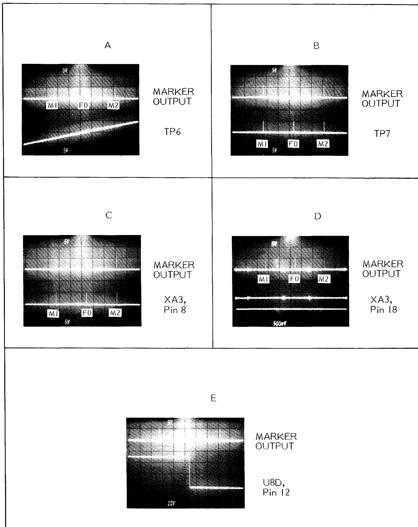
A3 Marker Generator PCB Waveforms (part of Figure 7-40)
