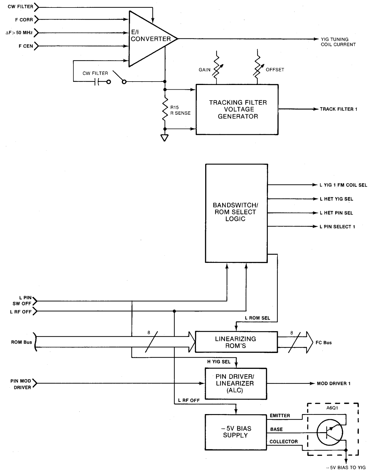
Figure 7-65. Assy 7007-4 YIG Driver PCB Overall Block Diagram
