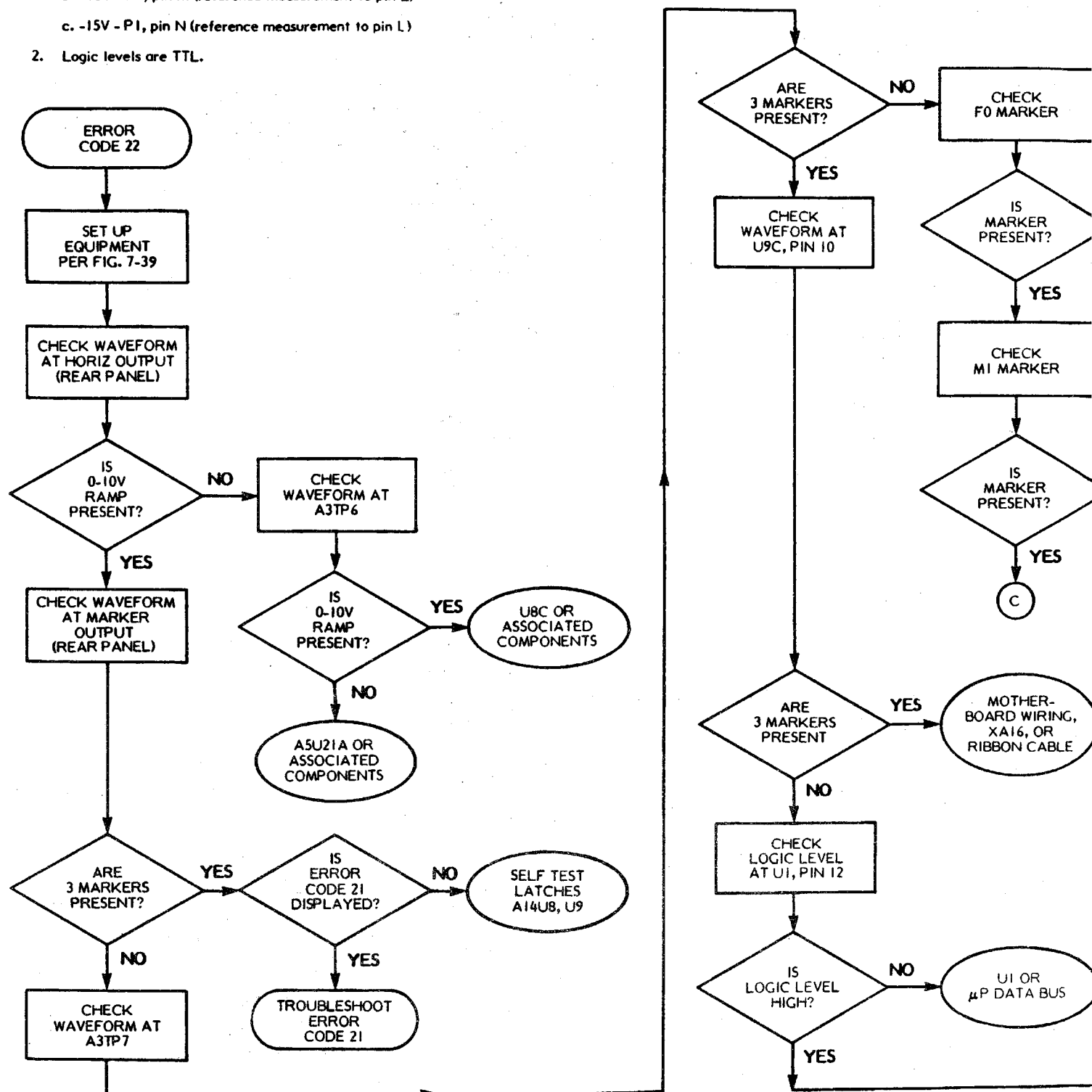
Figure 7-40. Error Code 22 Troubleshooting Flowchart (Sheet 1 of 3)
