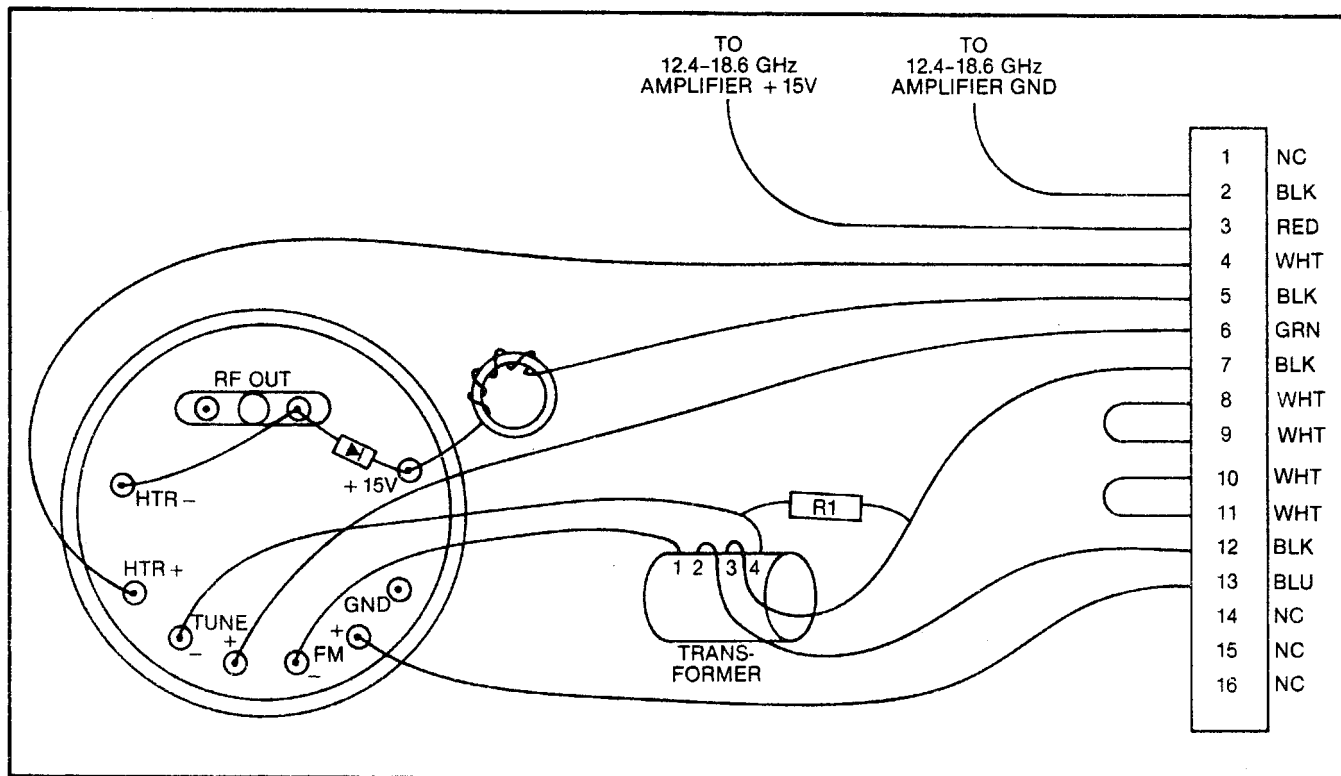
Figure 7-120. 6629A-40/6637A-40 A8 Avantek Oscillator Wiring Diagram
