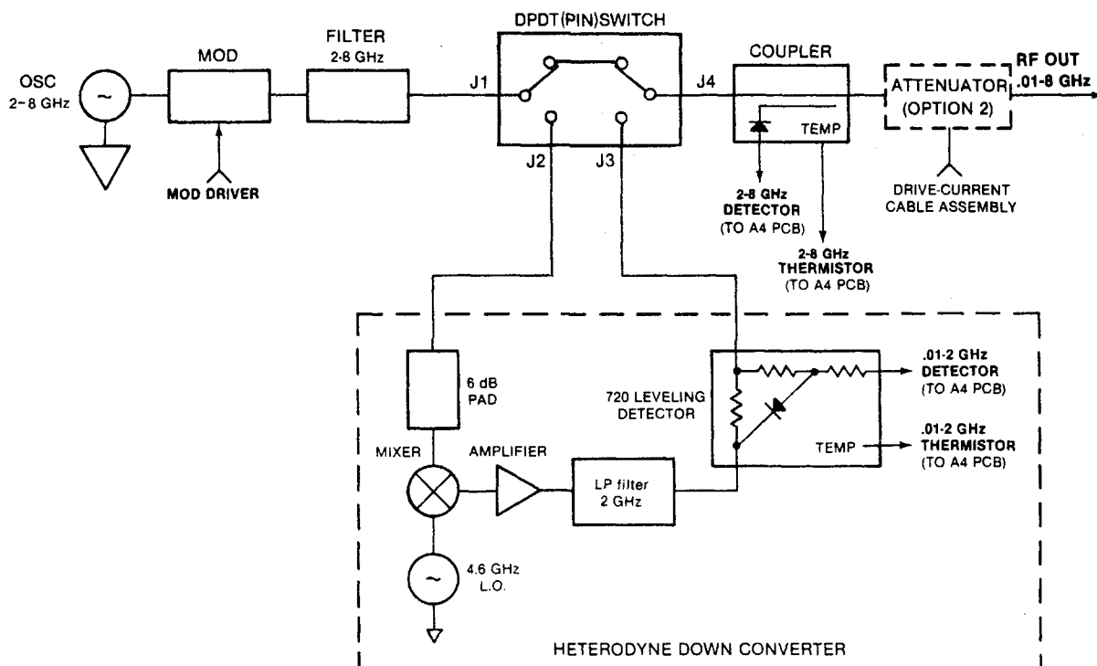
Figure 7-95. Model 6617A RF Components
