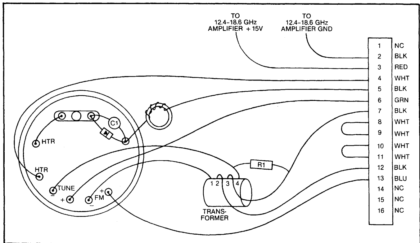
Figure 7-115. 6621A-40/6629A-40/6637A-40 A7 Avantek Oscillator Wiring Diagram
