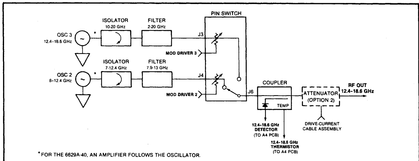
Figure 7-97. Model 6629A/6629A-40 RF Components
