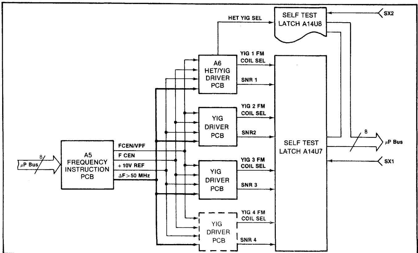
Figure 7-84. Error Codes 9 thru 14, Diagnostic (Self Test) Circuit
