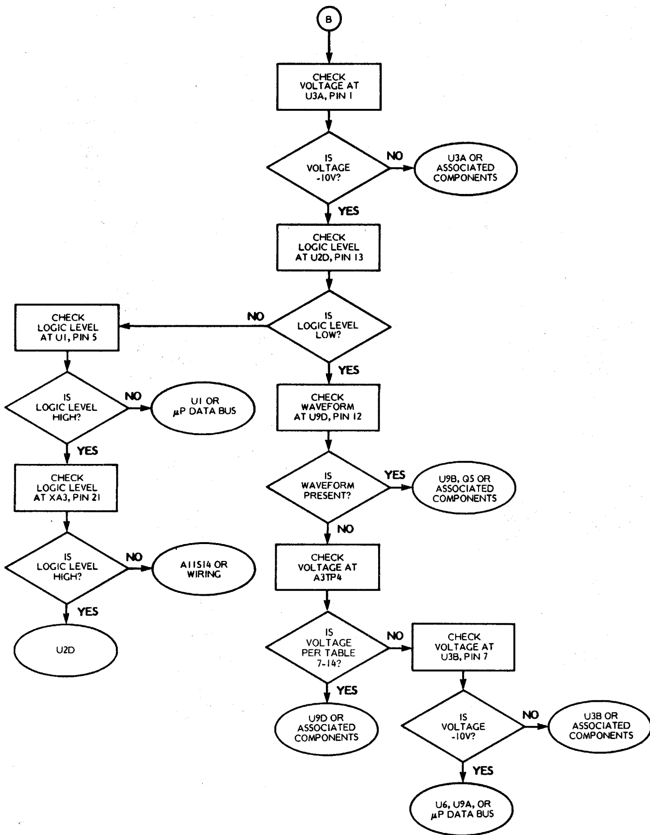
Figure 7-40. Error Code 22 Troubleshooting Flowchart (Sheet 2 of 3)
