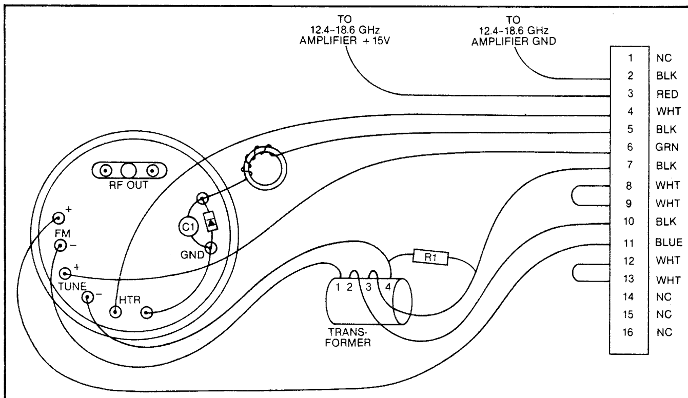
Figure 7-121. 6629A-40/6637A-40 A8 WJ Oscillator Wiring Diagram
