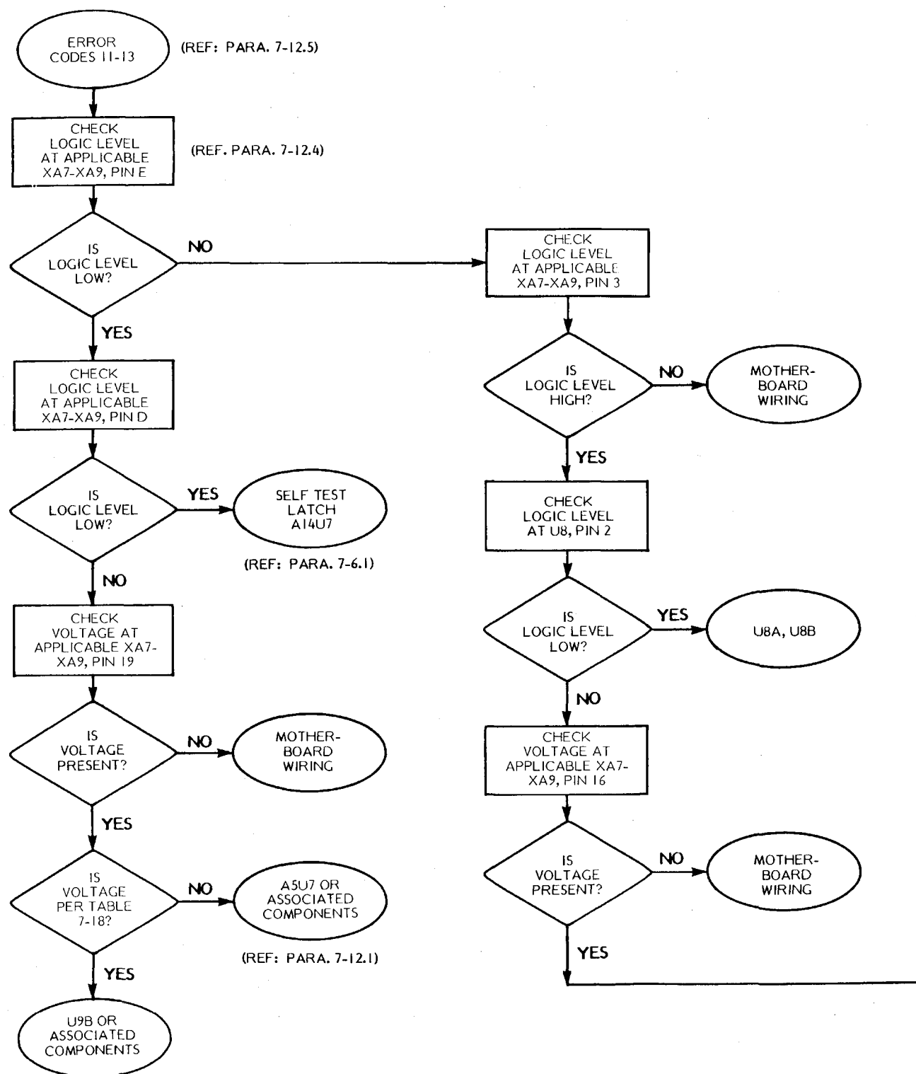
Figure 7-87. Error Code 11 Troubleshooting Flowchart
