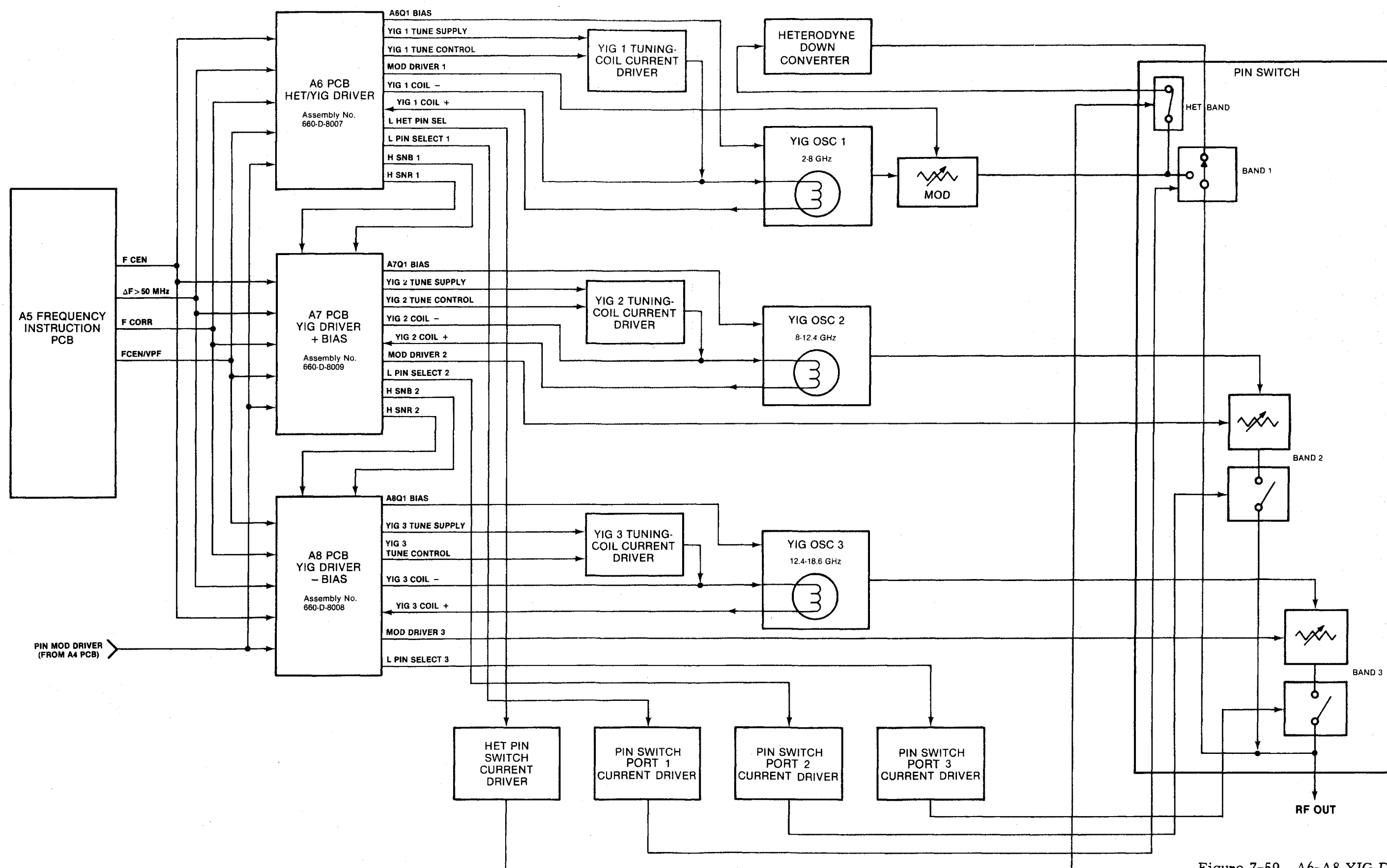
Figure 7-59. A6-A8 YIG Driver PCBs Overall Block Diagram
