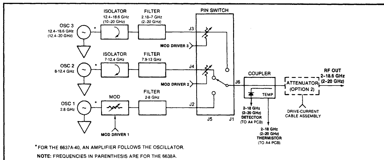
Figure 7-98. Model 6637A/6637A-40/6638A RF Components
