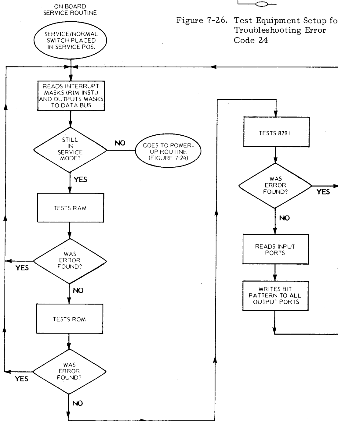
Figure 7-27. A1 PCB On-Board Service Routine
