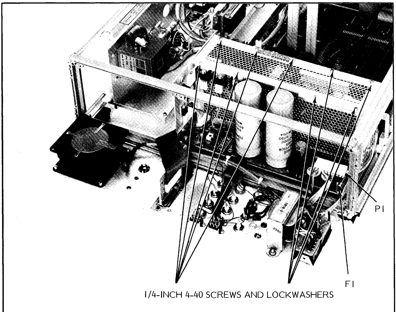
Figure 7-5. 6600A Series Programmable Sweep Generator, Rear Quarter Panels and Assemblies
