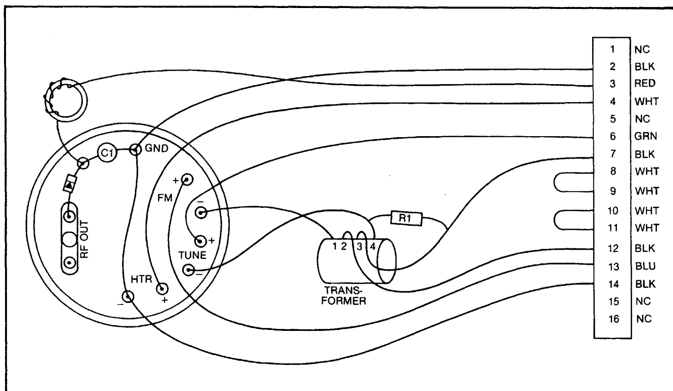
Figure 7-123. 6653A/6659A A8/A9 Avantek Oscillator Wiring Diagram
